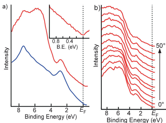
Figure 3. a) Angle-integrated photoemission spectra of 100–300 nm (blue) and 1.5–2.0 \mu\text{m} (red) porous graphene samples measured by a He II \alpha resonance line ( h\nu = 40.814 eV) at room temperature. The inset shows the angle-integrated PES spectrum near the Fermi level divided by the Fermi–Dirac function convoluted with the instrumental energy resolution. b) Angle-resolved PES spectra of nanoporous graphene with pore sizes of 1.5–2.0 \mu\text{m} .
